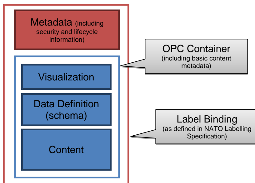
Figure 2: Submission Information Package structure
